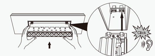
Retractable mechanism for easy maintenance.
