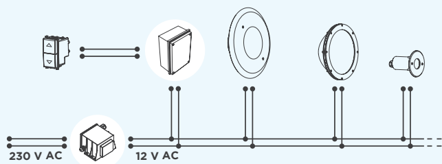
PLC with buttons wiring diagram
