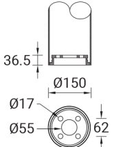
Mounting detail
