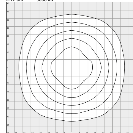
MR symmetrisch (150.400.ltd) LPH: 6m 9000 lm
