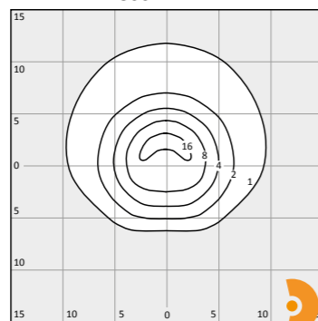
HS asymmetrisch (120.110.ldt) LPH: 4m 1800 lm
