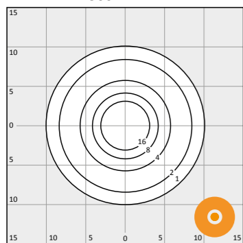
HS symmetrisch (120.100.ldt) LPH: 4m 2500 lm
