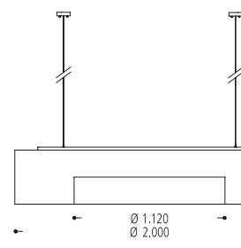
33.667.15-3717 6 x TC-L 2G11 55 W
